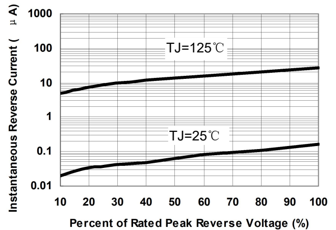
Fig.2-Typical Reverse Characteristics
